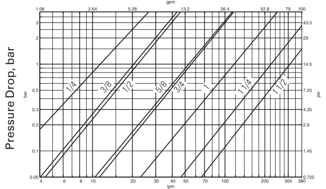
Gallons Per Minute Flow Test Fluid: MIL-H-5606 Oil at 100°F
